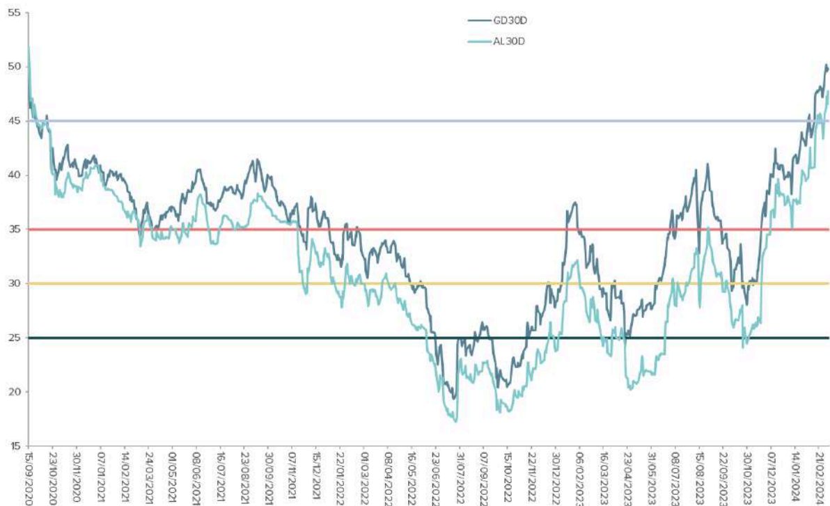
AL30D y GD30D Clean vs Recovery Value
